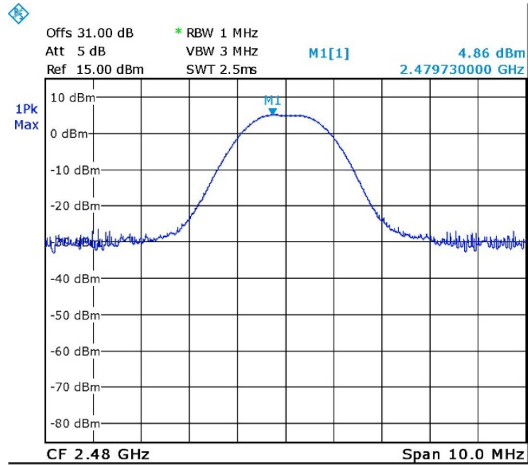
Figure 7. High Channel, BLE
