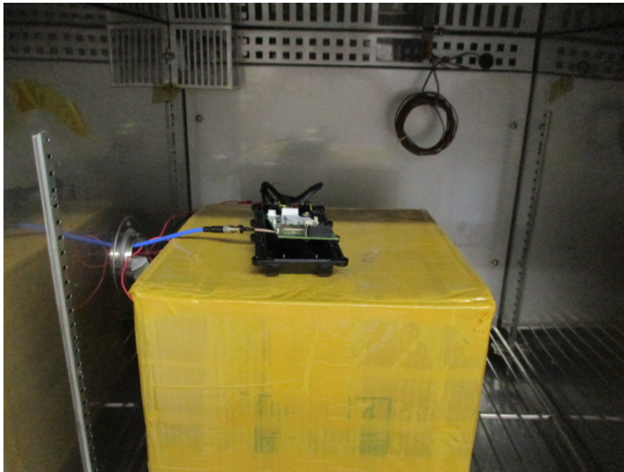
Figure 19. RF Output Power Test
