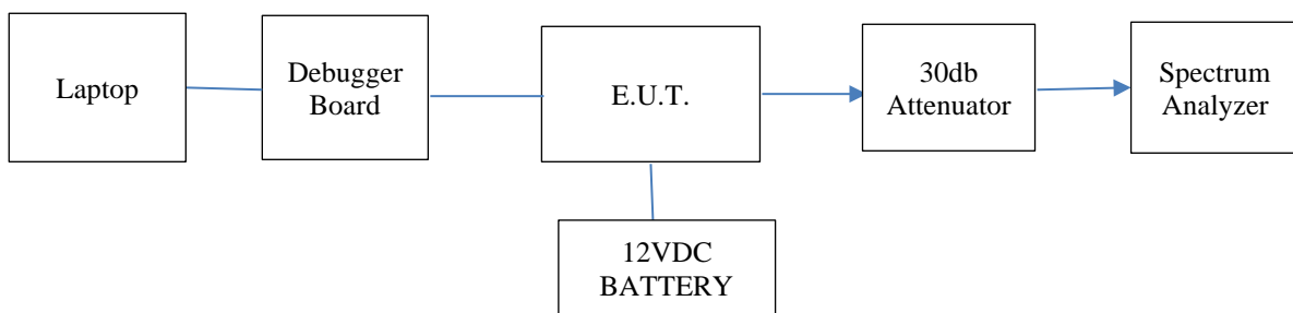
Figure 1. Configuration of Tested System - Conducted
