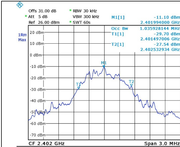
Figure 8. Low Frequency, BLE Mode
