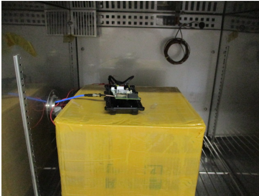
Figure 21 Transmitter Unwanted Emission in the OOB Domain
