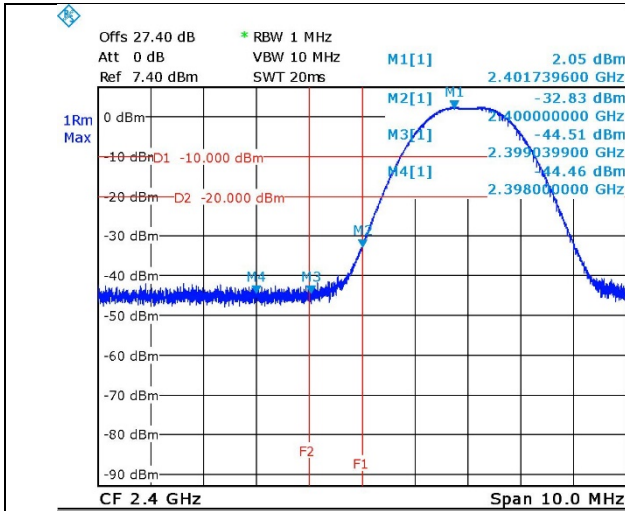
Figure 10. Low Frequency, BLE Mode
